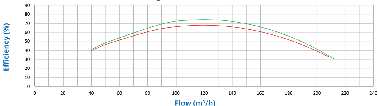
Hydraulic Performance
