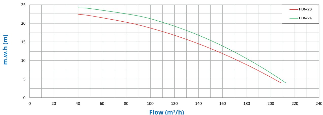
Characteristics curve
