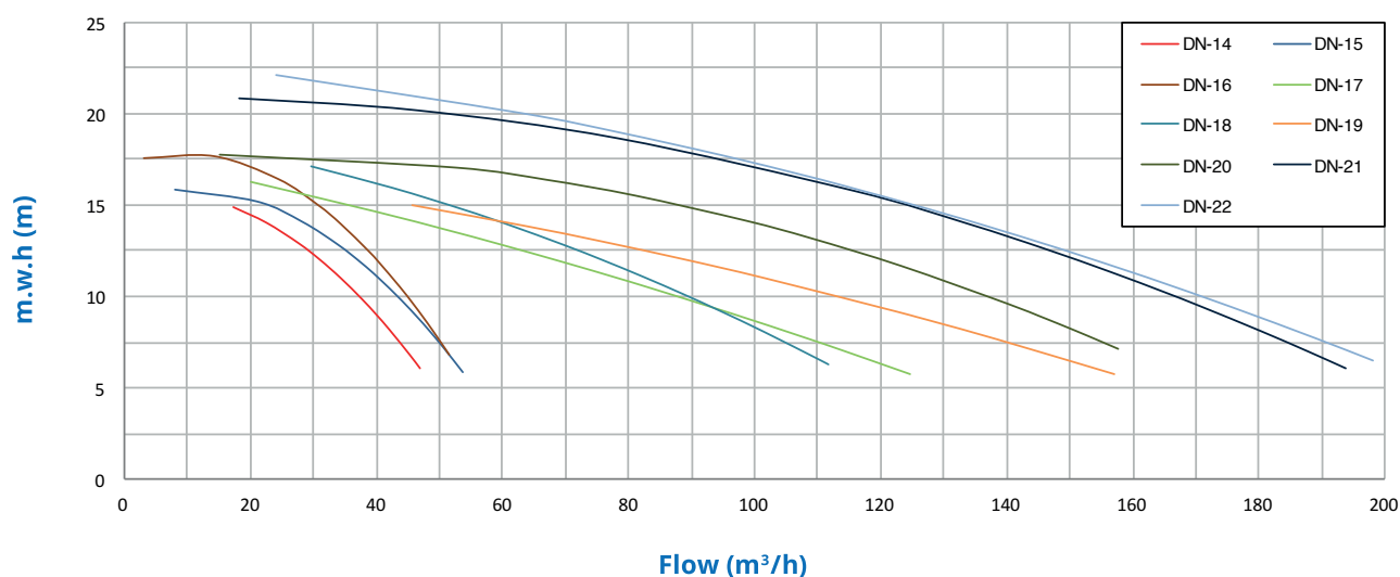
Characteristics curve
