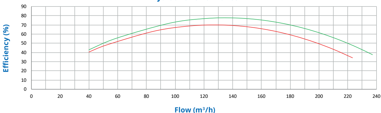
Hydraulic Performance
