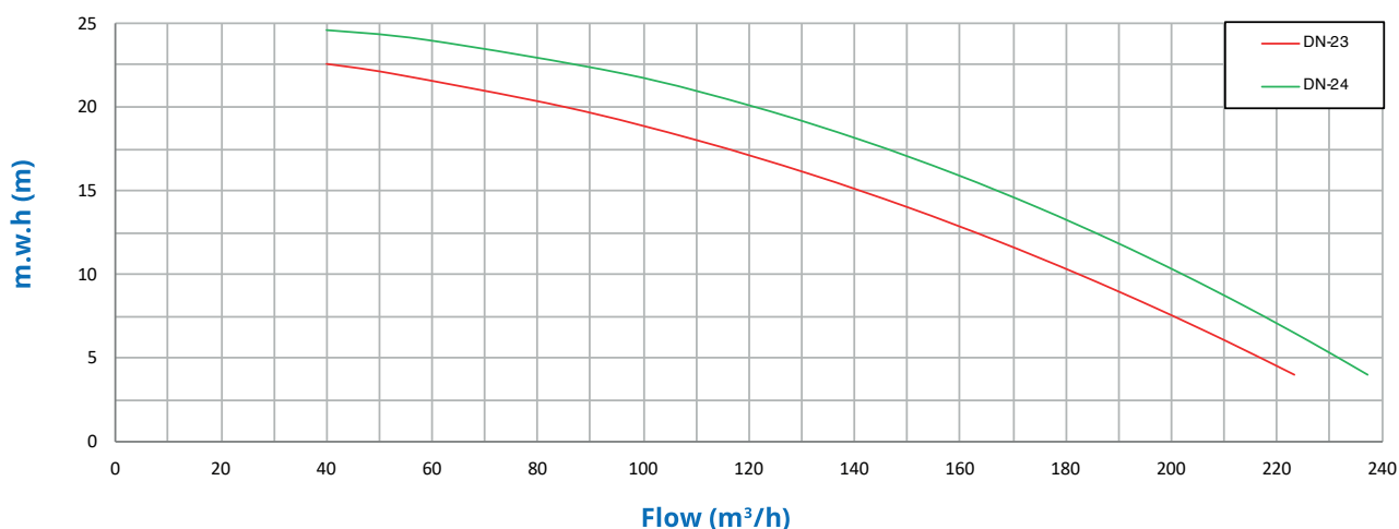
Characteristics curve
