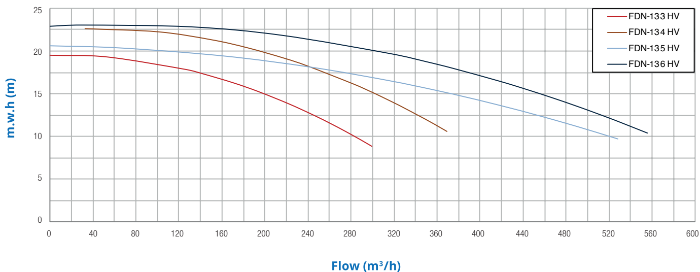
Characteristics curve
