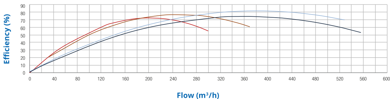
Hydraulic Performance
