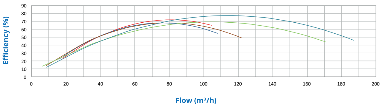
Hydraulic Performance
