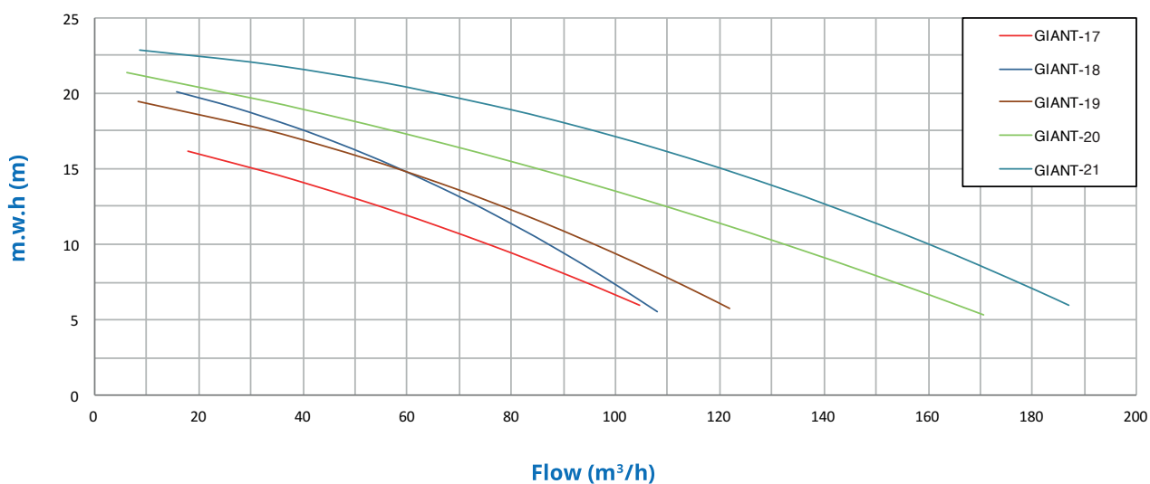
Characteristics curve
