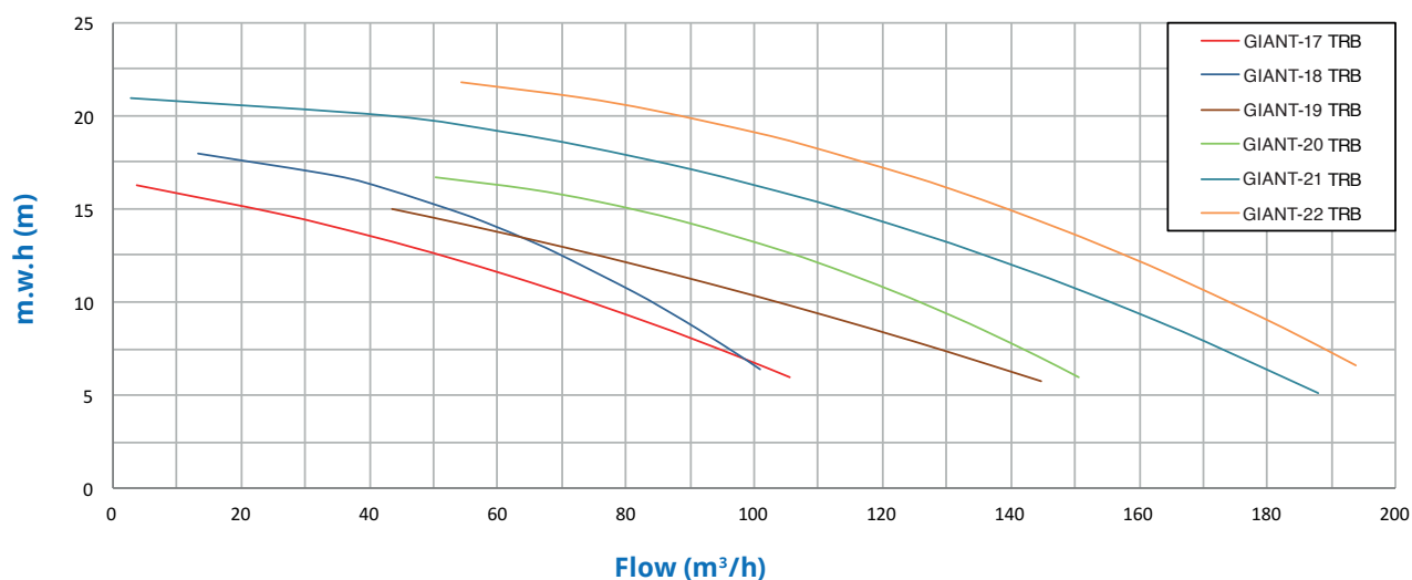
Characteristics curve
