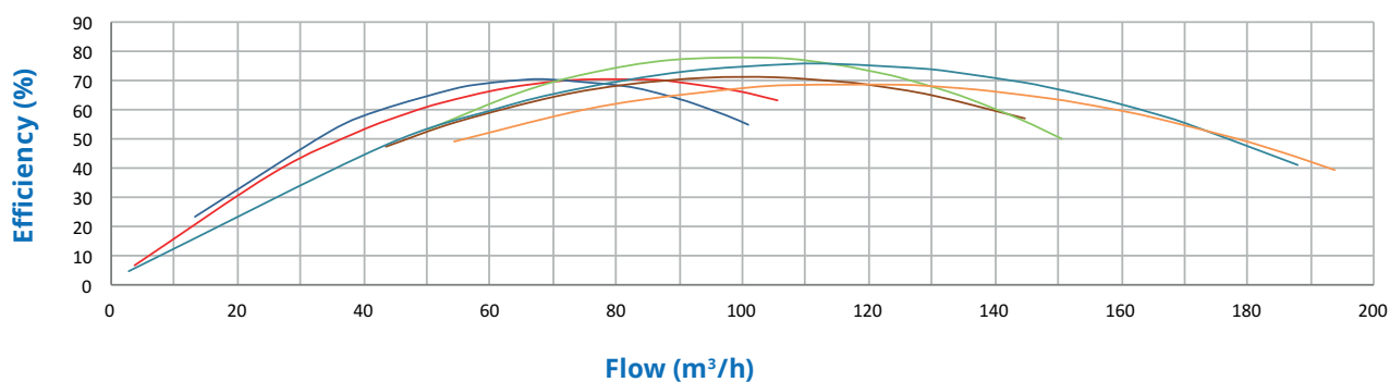
Hydraulic Performance
